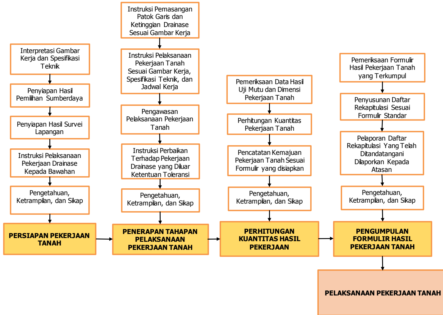
Gambar 1. Diagram Proses
