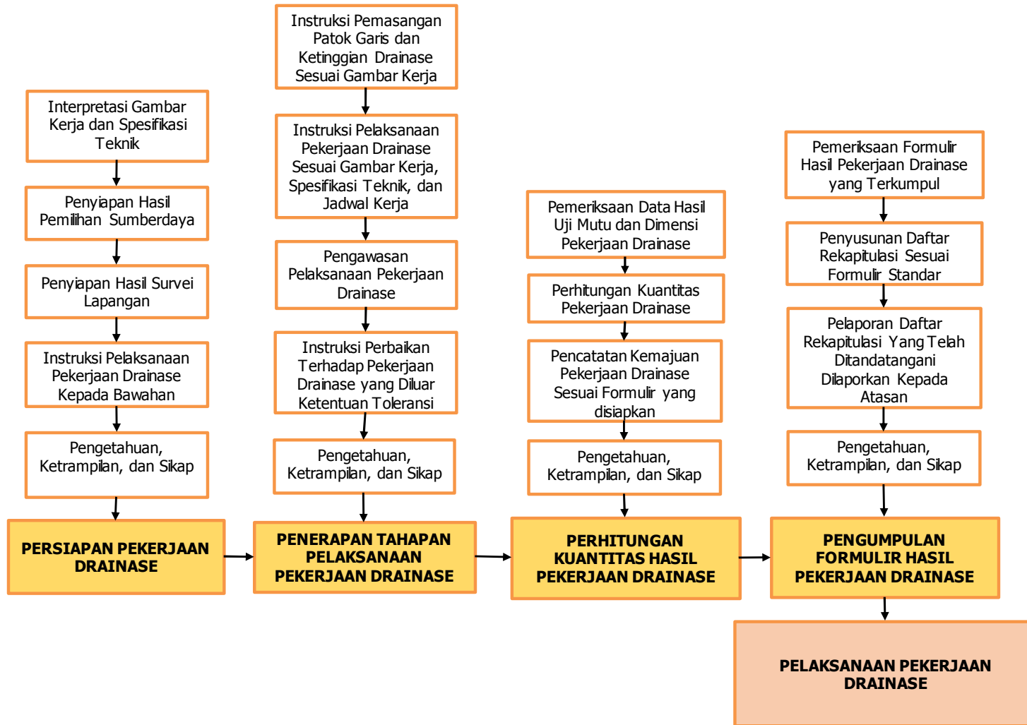
Gambar 1. Diagram Proses
